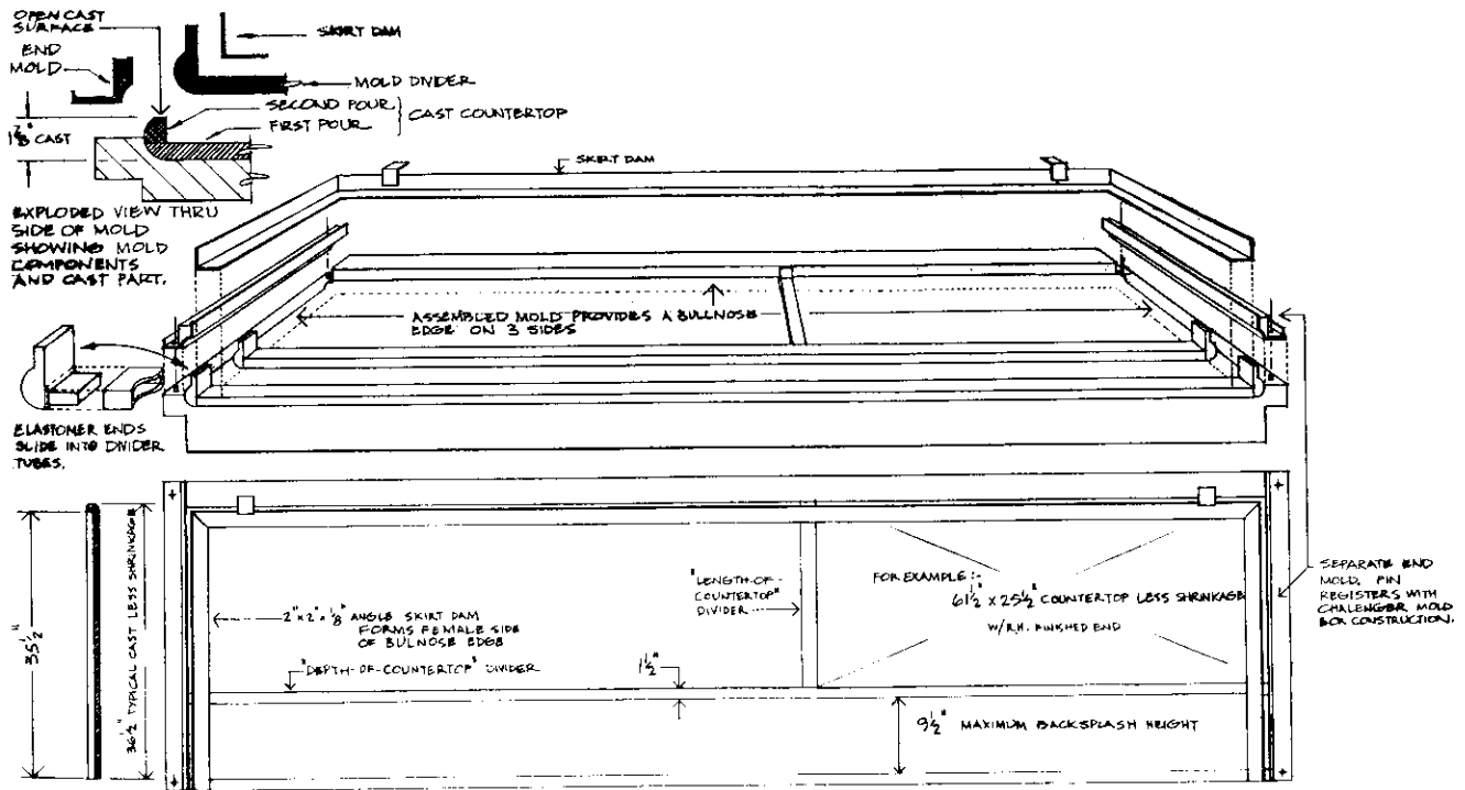
PLAN VIEW OF THE MOLD COMPONENTS SET UP TO PRODUCE A SPECIFIED COUNTERTOP AND BACK SPLASH.
